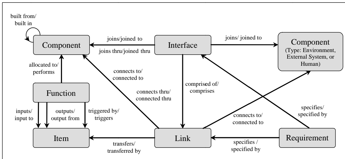
Figure 14 External Interface Definition
