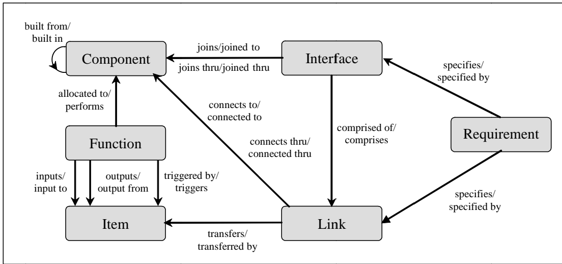
Figure 15 Internal Interface Definition
