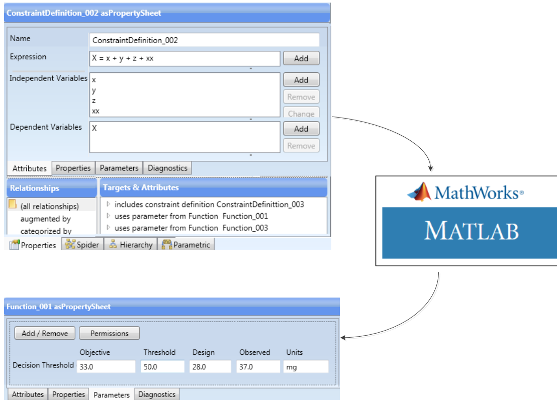
Figure 1 – MATLAB Constraint Solver Concept Graphic
